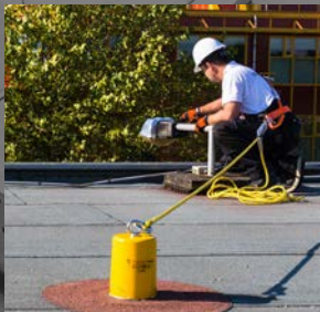
TEMPORARY HORIZONTAL LIFELINES
